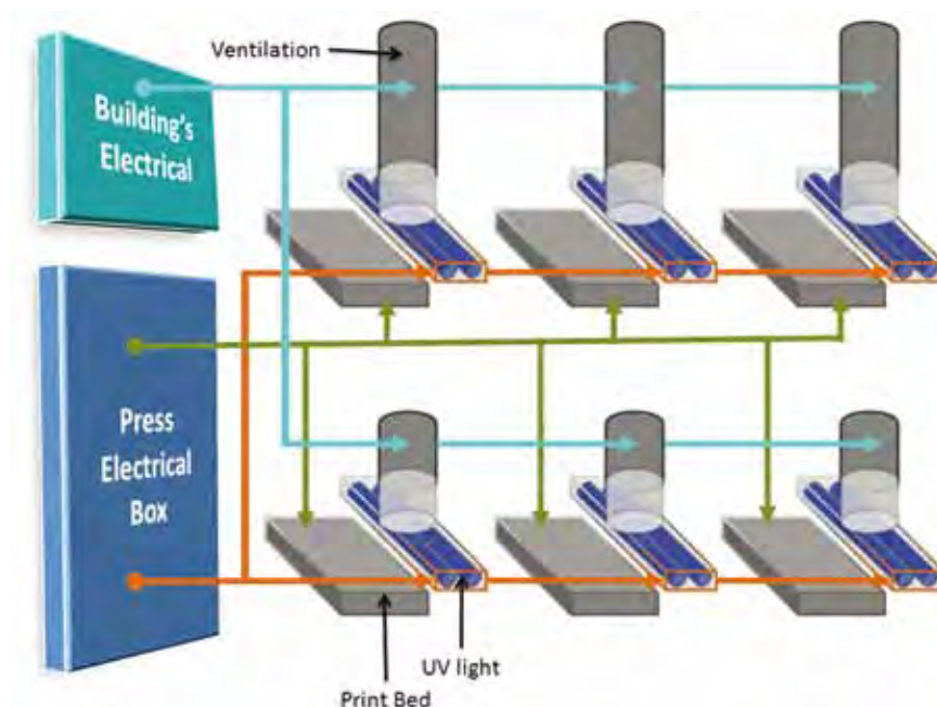
Diagram 1: the electrical supply for a 6-station in-line press using mercury vapour lamps
